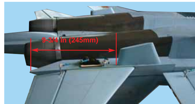
28C - Use 30 minute epoxy to glue the left ventral fin to the fuselage
