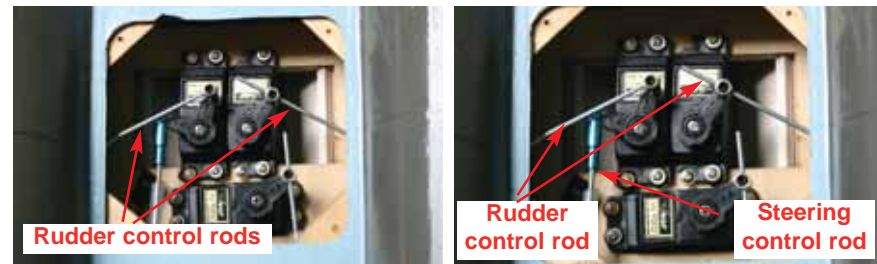
19C - With the servos and rudders at neutral, connect the clevises and then tighten the control horn set screws. 19D - Connect the nose gear steering control rod.
