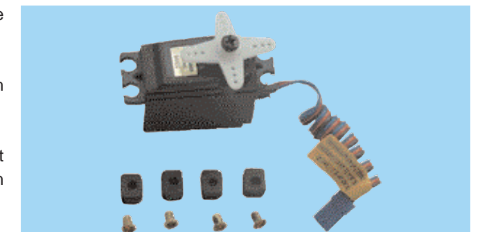
2A - Prepare the servos by fitting the rubber grommets & ferrules supplied with your servos
