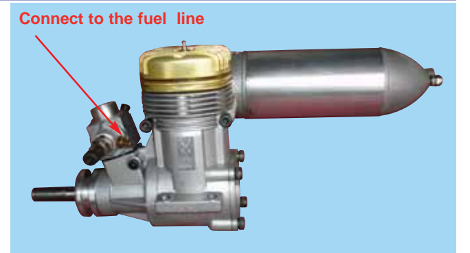
12A - .91 2 cycle engine. VMAX 91PRO shown
