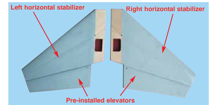
5A - Left and right horizontal stabilizers with pre-installed elevators
