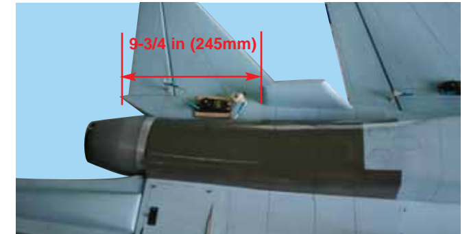
28B - Use 30 minute epoxy to glue the right ventral fin to the fuselage
