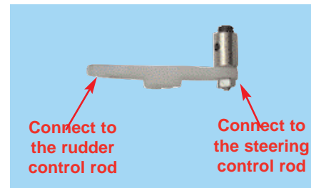
19E - Connecting the steering control rod to the servo arm. NOTE: In some market areas, the EZ connector shown has been replaced by a clevis.
