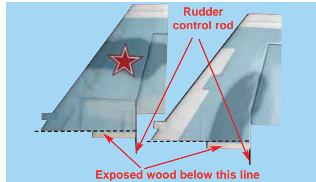
6A - Vertical stabilizer with pre-installed rudder and rudder control rod
