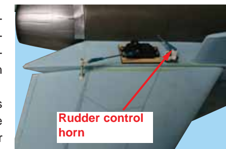
19A - Connect the 2 rudder control rods to the rudder control horns.
