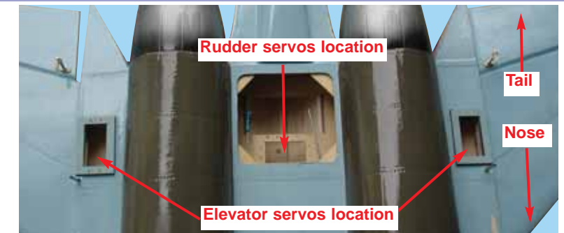
17A - Location of the 2 elevator, 2 rudder and throttle servos.
