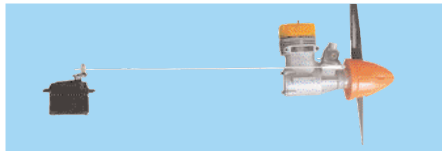
20B - The throttle servo controls the engine throttle using the throttle control rod
