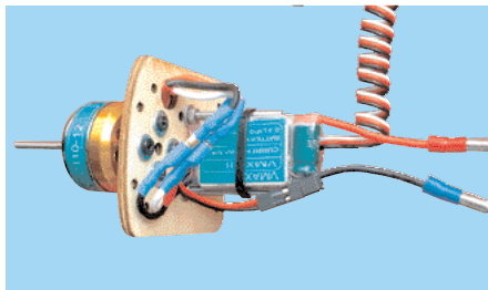
11E - Secure the Electronic Speed Control to the restraining bolts using a tie wrap as shown
