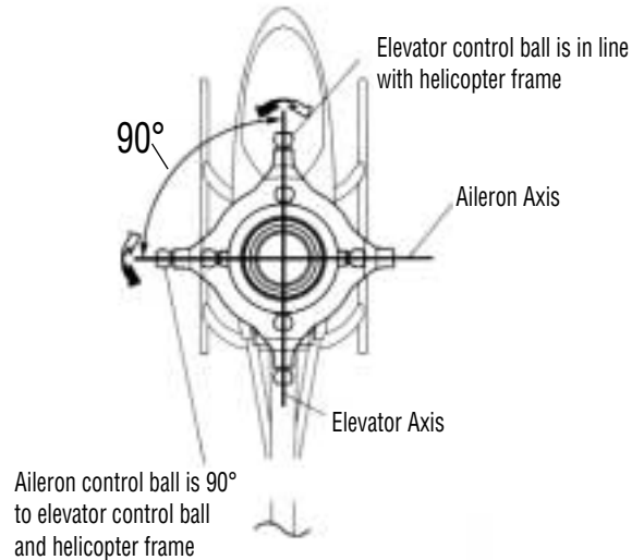
Standard "1 Servo" Swashplate System
