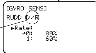
XP8103 with NEJ450, NEJ900 & NEJ3000 Gyros
