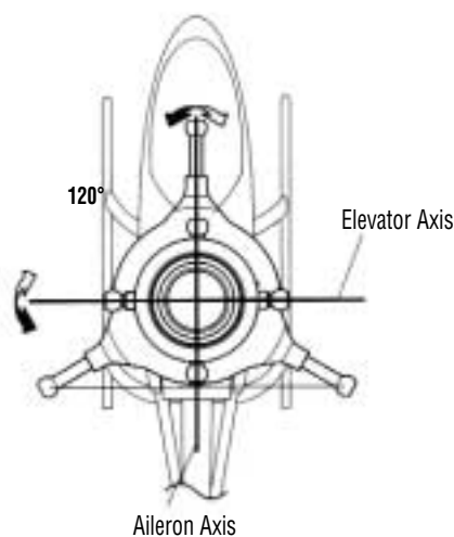
JR 120° 3 Servo CCPM Control System
