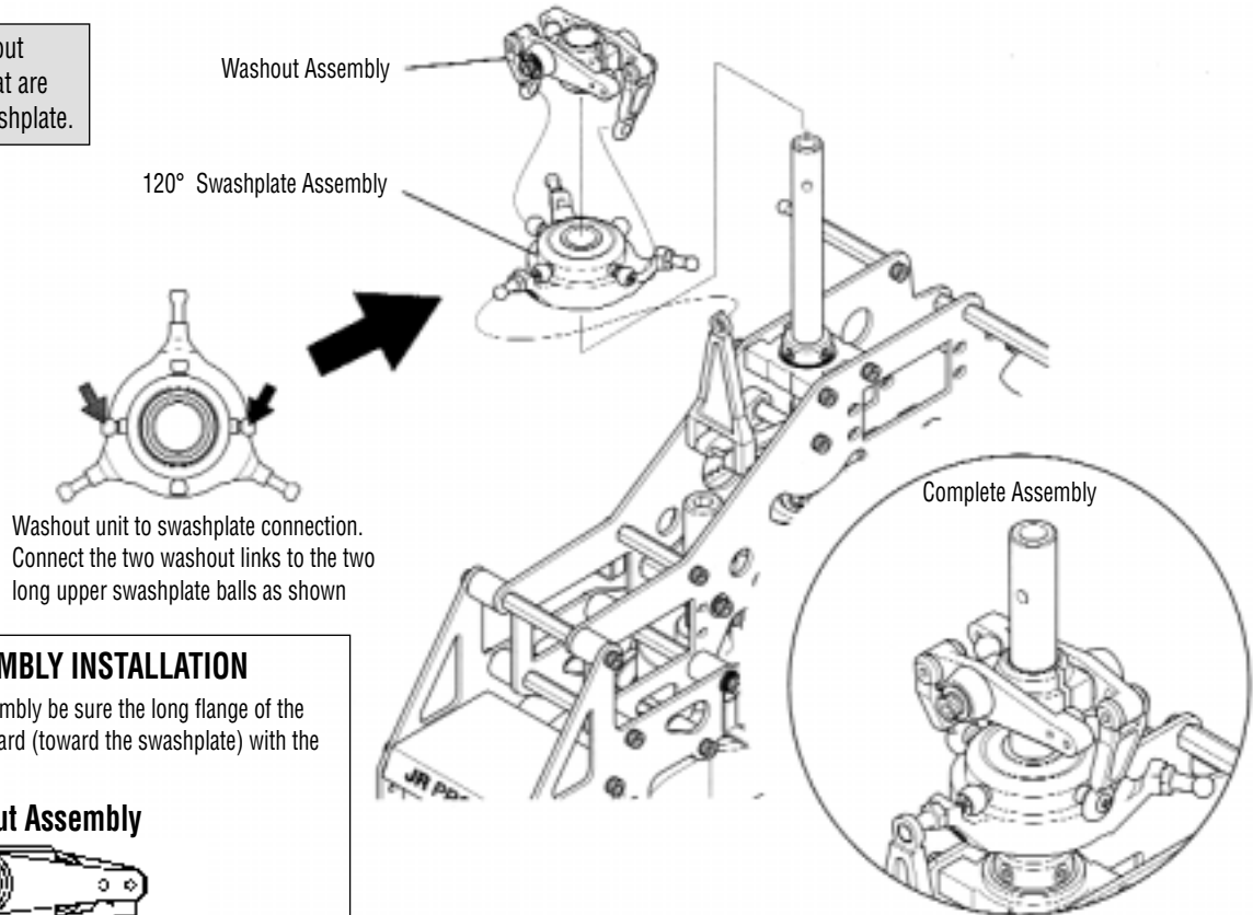
Long portion of mixing base flange must face downward.
