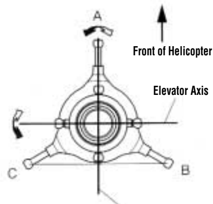
JR 120° CCPM Control System
