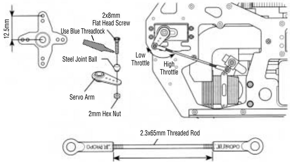
JR System/Webra .35 Engine or MDS .38 Heli Engine
