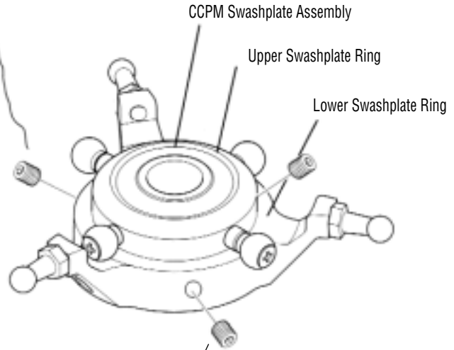
4x4mm Swashplate Adjusting Screws (Caution: Do not overtighten!)
