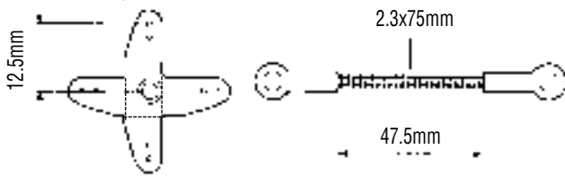
JR System/Webra .35 Engine or MDS .38 Heli Engine
